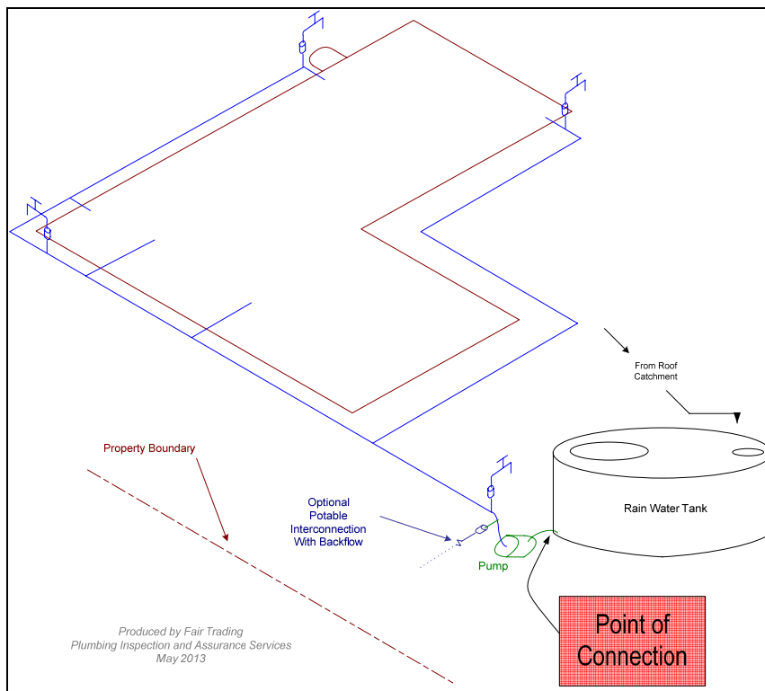
Diagram 2 - Point of connection: rainwater tank
